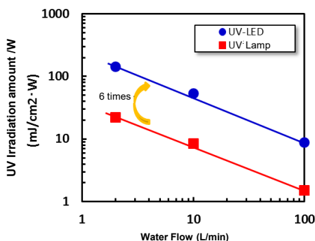
Reduction Equivalent Dose per UVC power of 1W
