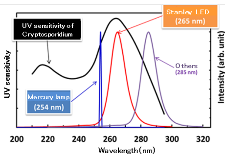
Emission spectrum and UV sensitivity of Cryptosporidium
