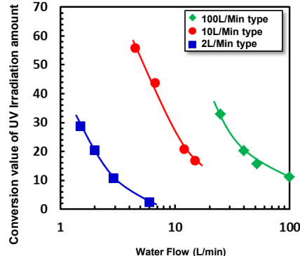
Reduction Equivalent Dose of E. coli Phage MS2
