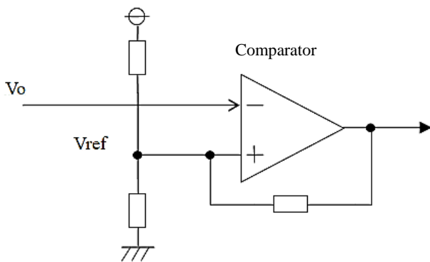
Fig.13 Comparator circuit
