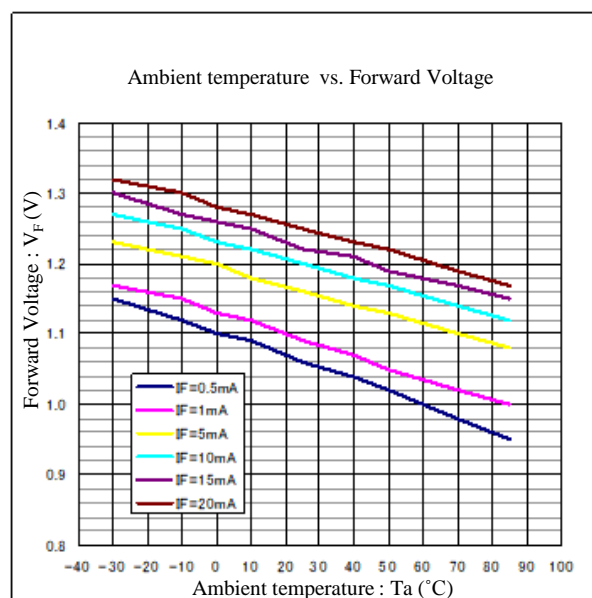
Fig.3 Forward voltage characteristics of KU163 /infrared LED
