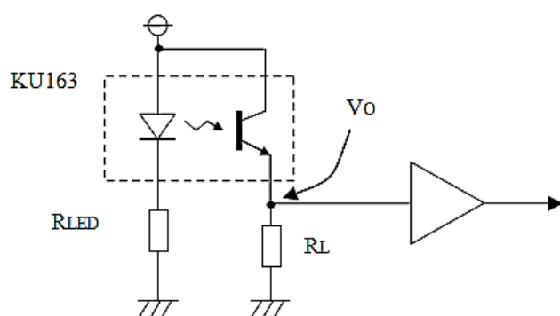
Fig.11 Applied circuit example
