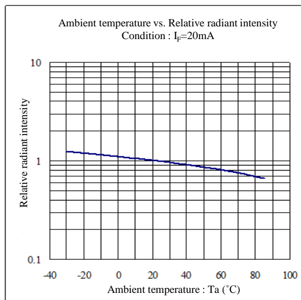
Fig.2 Output characteristics of KU163/infrared LED
