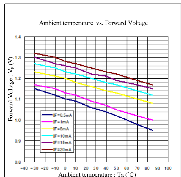
Fig.3 Forward voltage characteristics of KU163 /infrared LED
