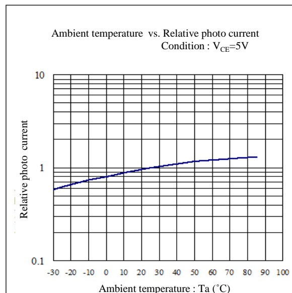
Fig.6 Photo current characteristics of KU163/phototransistor
