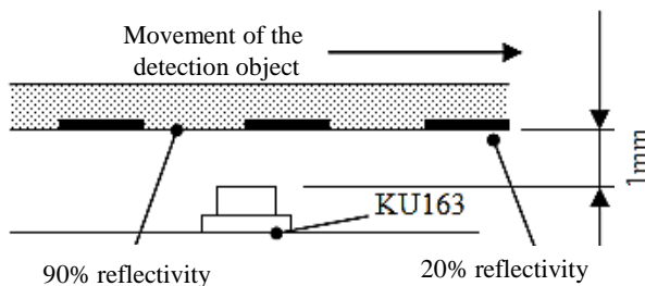
Fig.10 Application example
