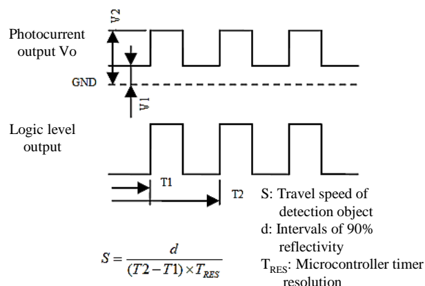
Fig.12 Speed detection
