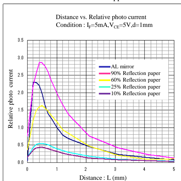
Fig.9 KU163 distance vs. photocurrent characteristic
