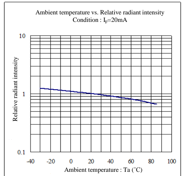
Fig.2 Output characteristics of KU163/infrared LED
