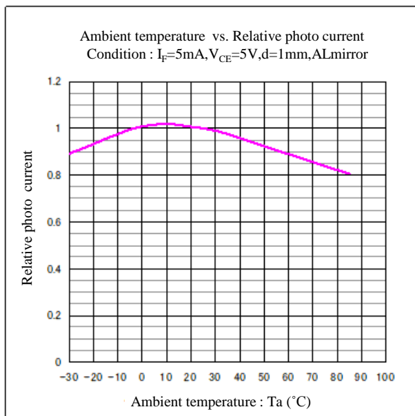
Fig.8 KU163 photocurrent characteristic
