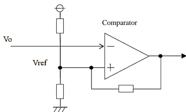
Fig.13 Comparator circuit
