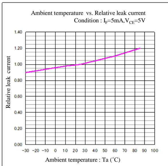
Fig.7 KU163 leak current characteristic
