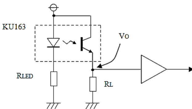
Fig.11 Applied circuit example
