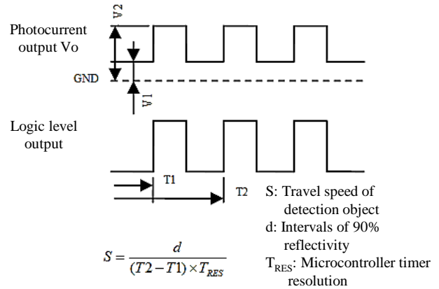
Fig.12 Speed detection
