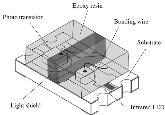
Fig.1 Structure of KU163
