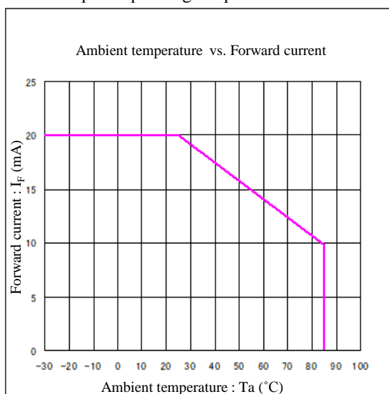
Fig.4 Derating characteristics of KU163/infrared LED
