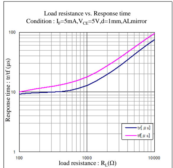
Fig.14 KU163 response characteristic
